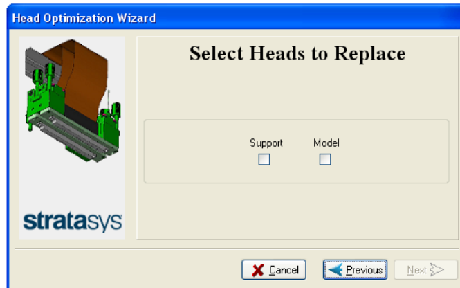
Figure 6-83 Head selection
