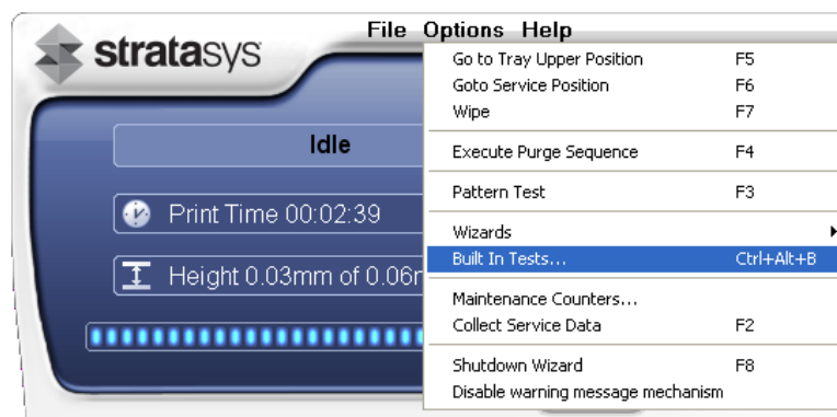
Figure 6-146 Selecting Built-In Tests from the Options menu
