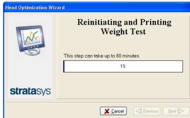
Figure 6-72 Wizard progress
