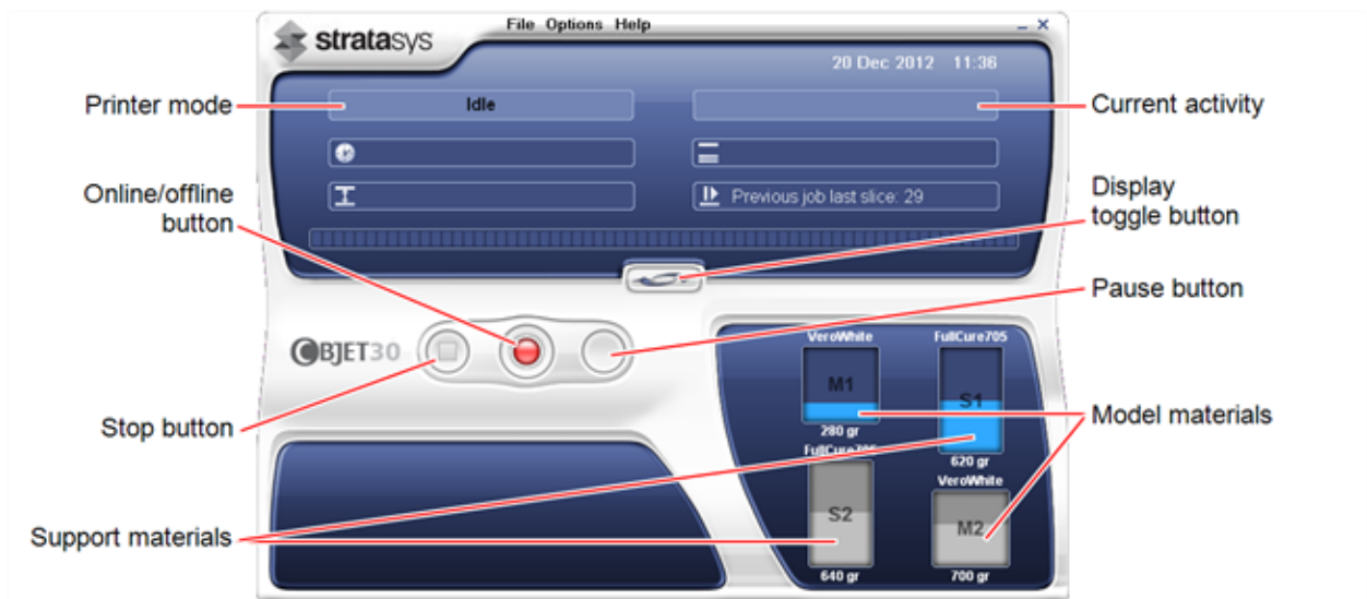
Figure 6-3 Printer interface
